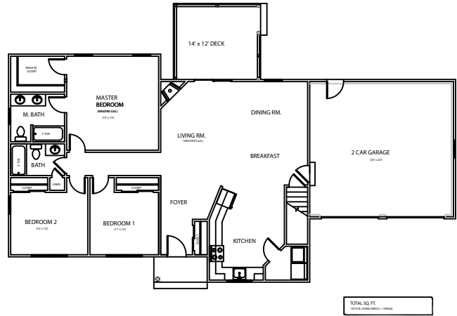
FIRST FLOOR PLAN SCALE 1/4" = 1'-0"
