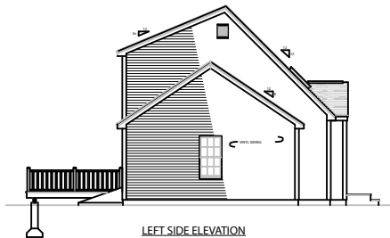
LEFT SIDE ELEVATION SCALE 1/4" = 1'-0"
