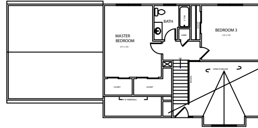
SECOND FLOOR PLAN SCALE: 1/8" = 1'-0"
