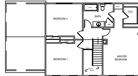
SECOND FLOOR PLAN SCALE 1/4" = 1'-0"
